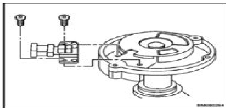
Figure 40. Camshaft Position Sensor Remove/Install
