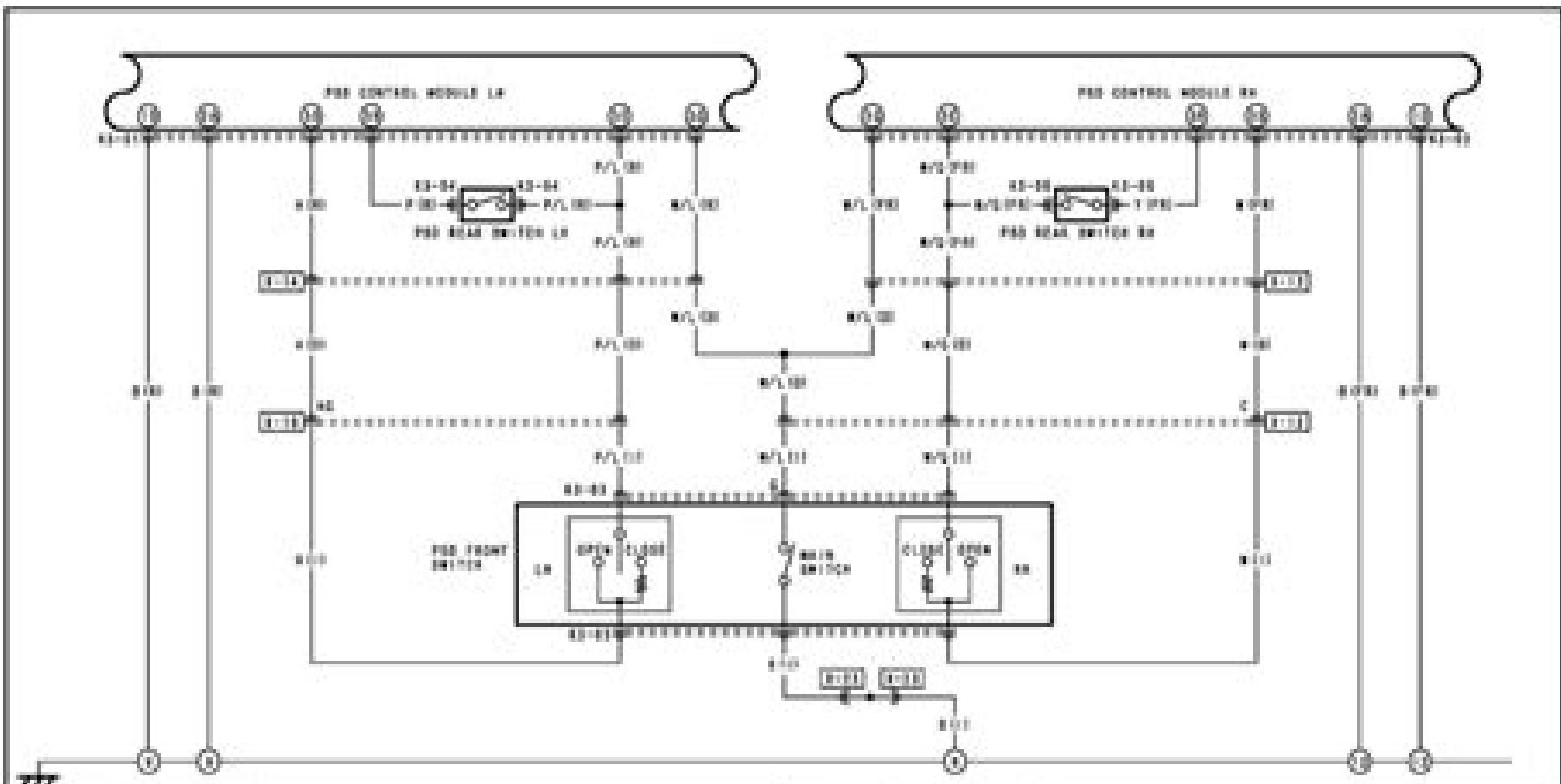
10-01 PED CONTROL MODULE LA W/P
