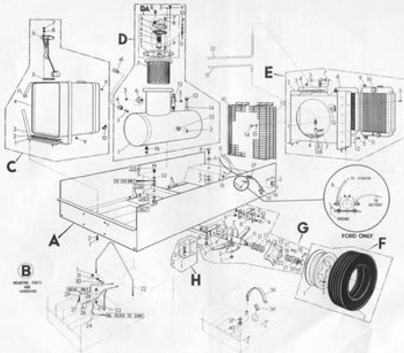
FIGURE 2 BASIC MACHINE AND AXLE ASSEMBLY Reference Dwg. AD-2
