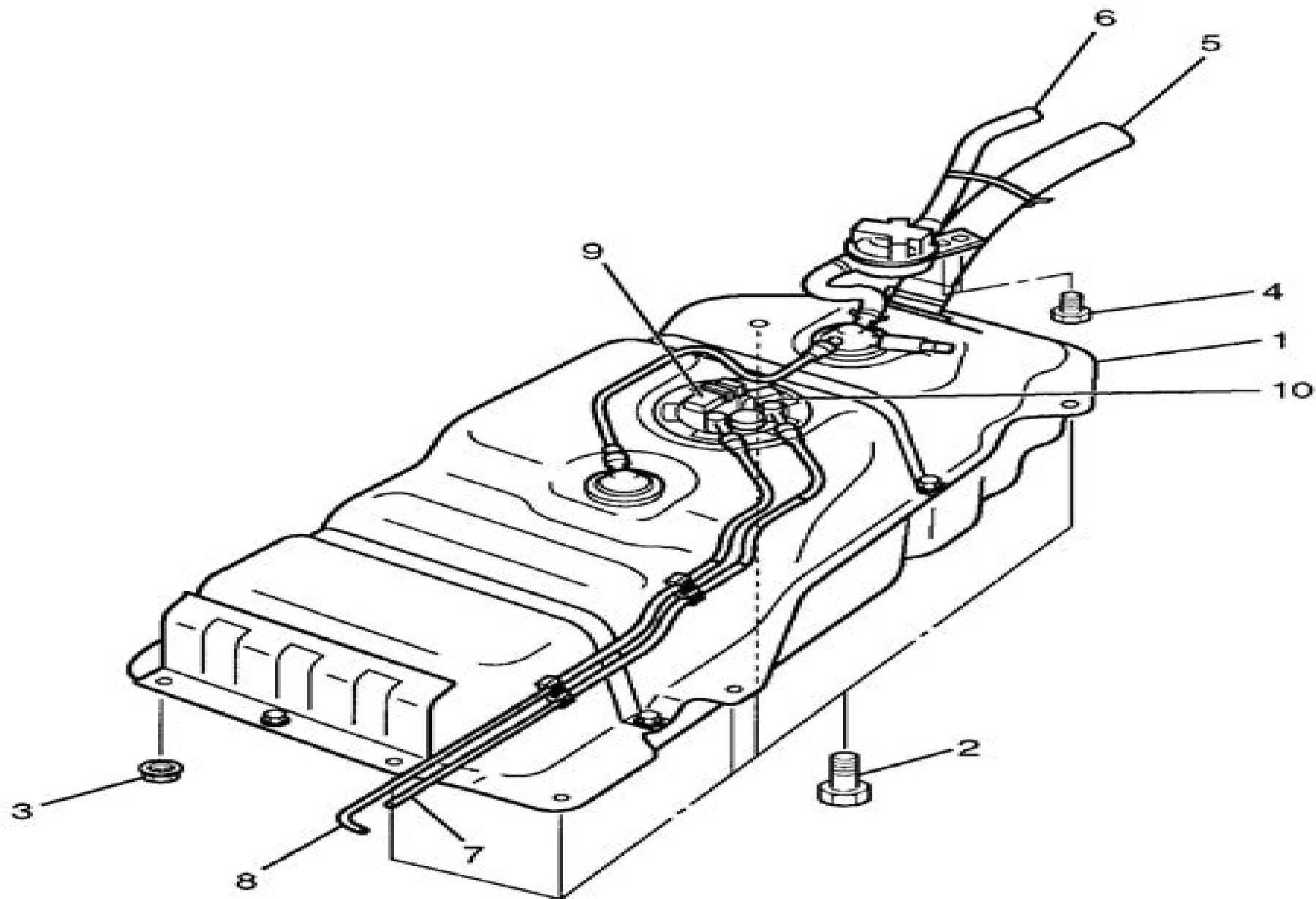
Fuel Tank (3.2L)
