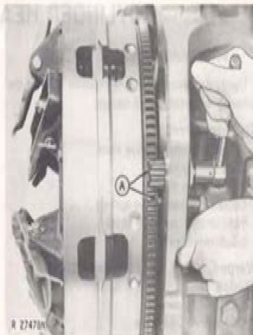
Fig. 3-Setting "TDC"
