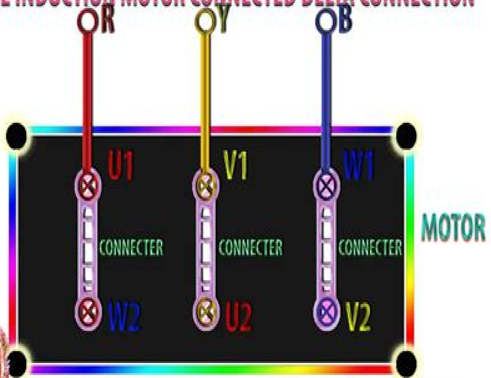
PHASE INDUCTION MOTOR CONNECTION DIAGRAM
