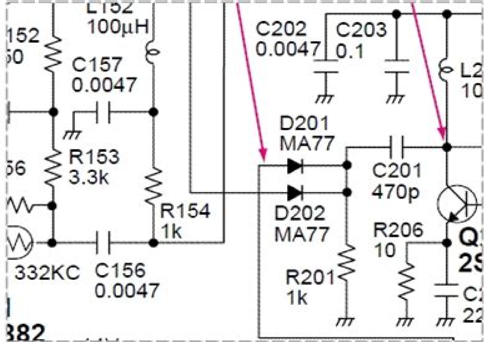
Preview: ICOM IC-718 schematic diagram
