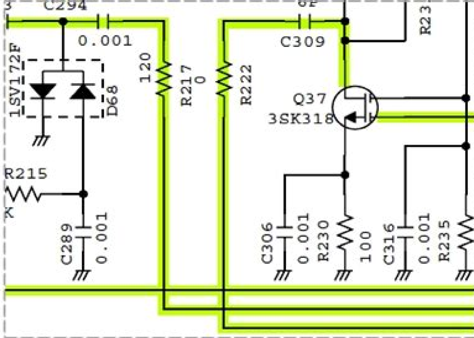
Preview: ICOM IC-2820H schematic diagram
