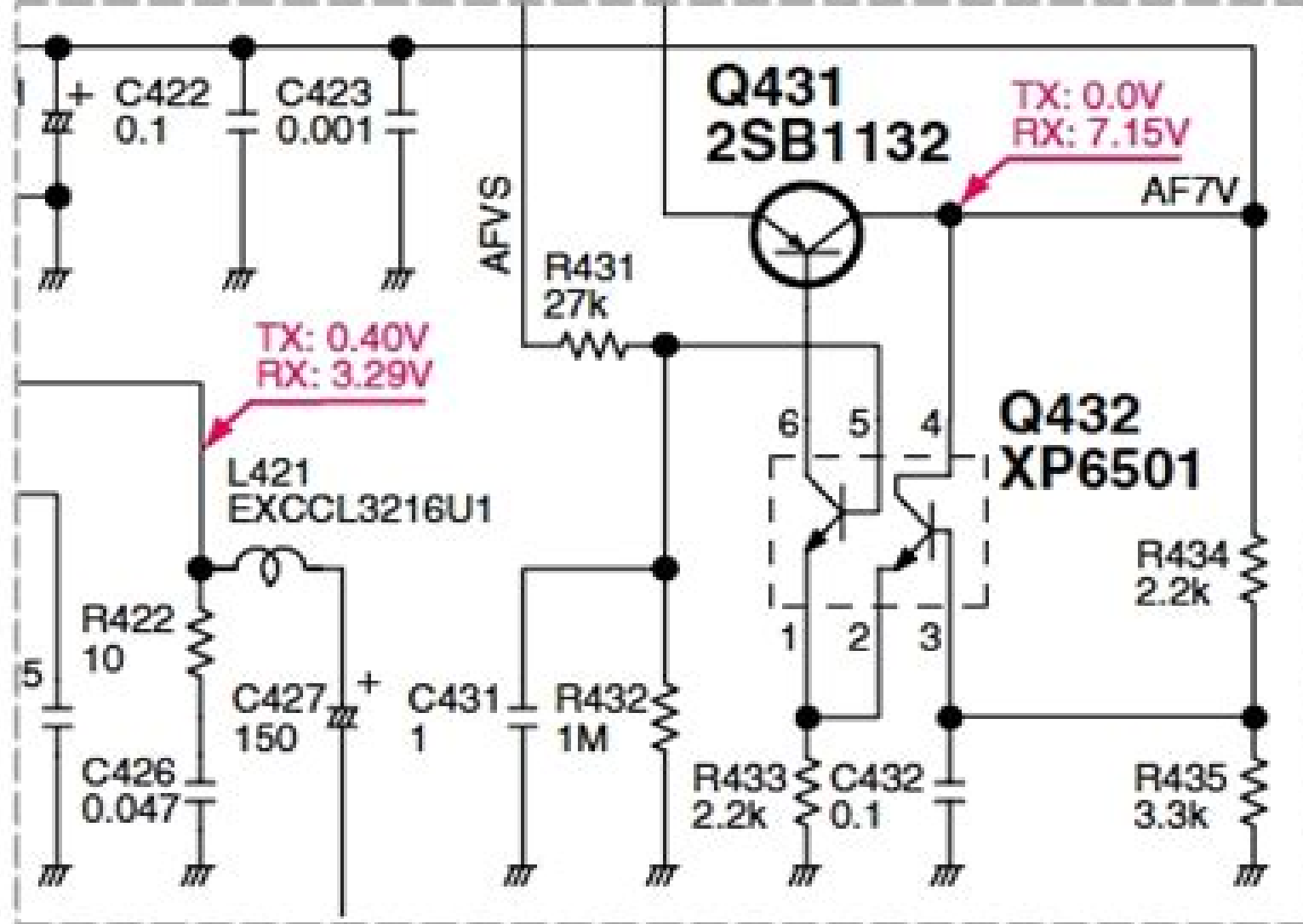
Preview: ICOM IC-M88 schematic diagram
