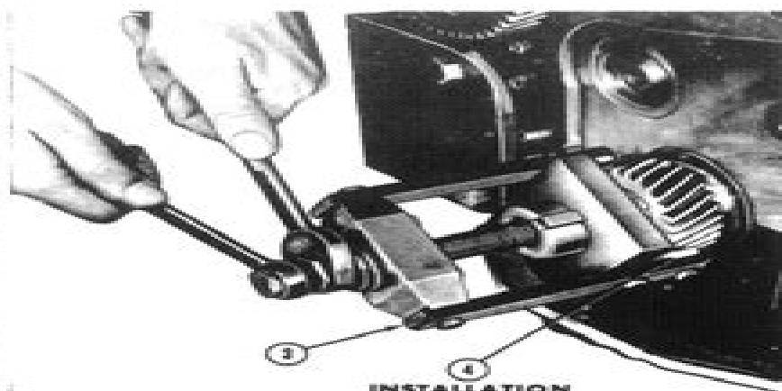
Figure 28 Removing and Installing Crankshaft Gear
