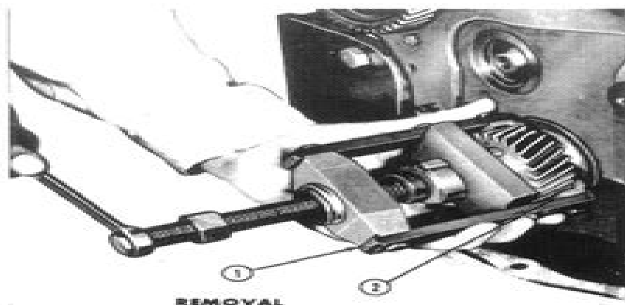
Figure 28 Removing and Installing Crankshaft Gear
