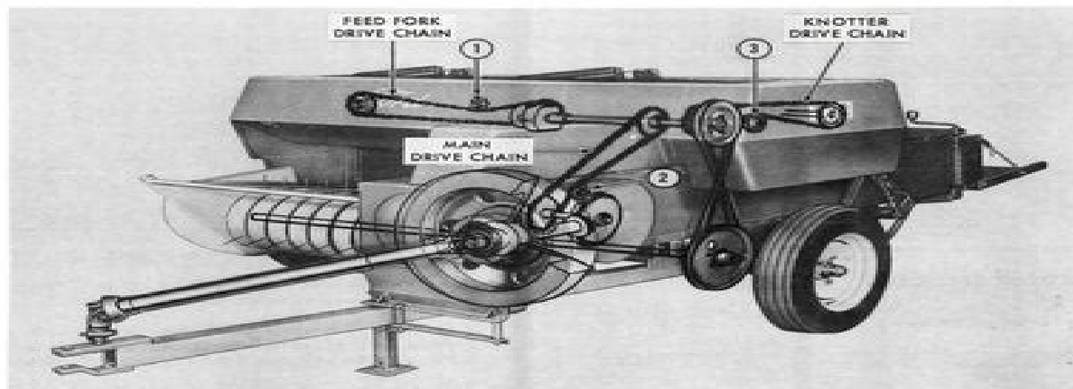
Figure 30 Adjusting Drive Chains
