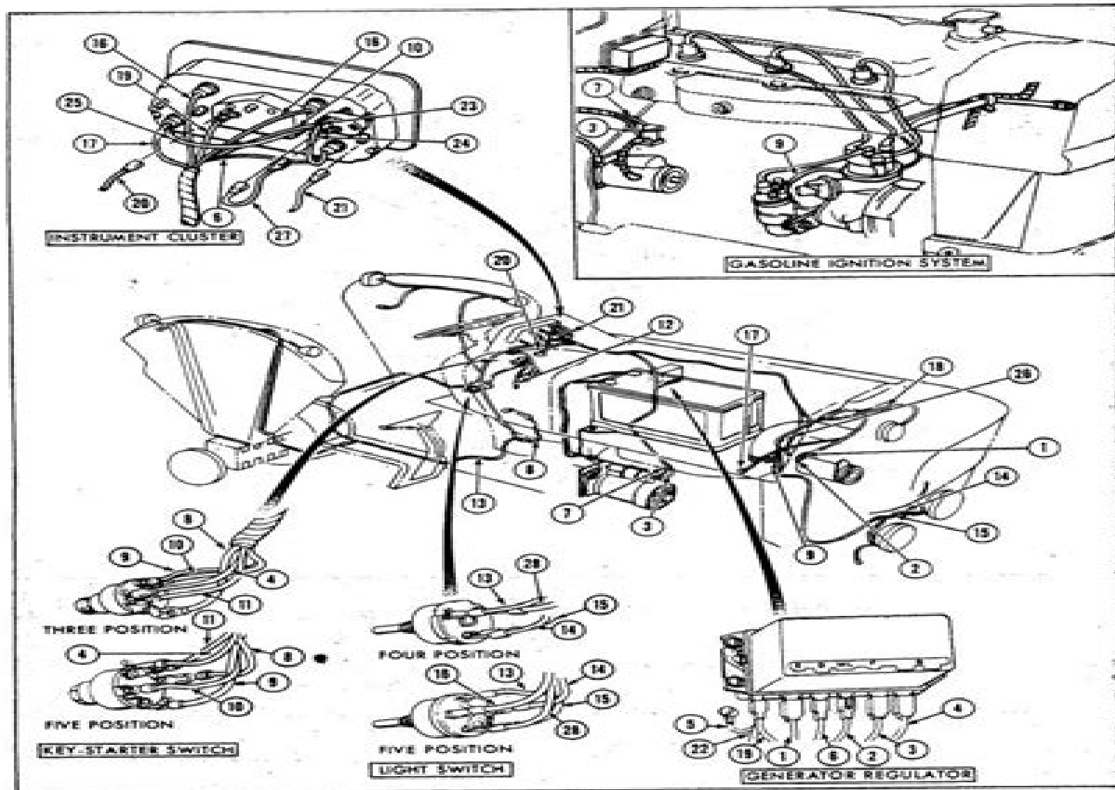
Figure 6 Circuit Descriptions—Tractors with "A" or "B" Prefixed Serial Numbers
