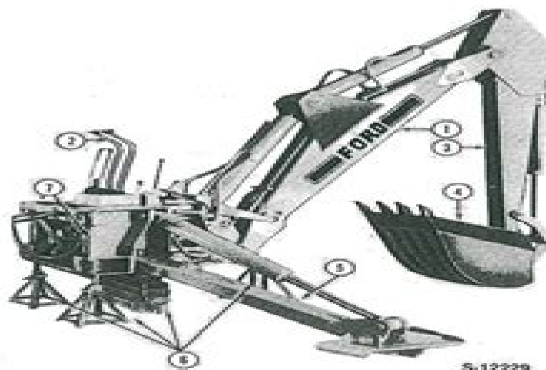
Figure 69 Backhoe Removed
