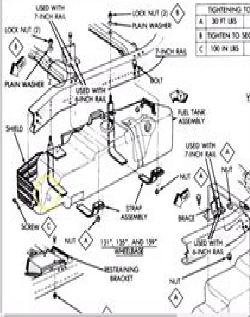
Fig. 1 Common components of the rear lower mounted fuel tank
