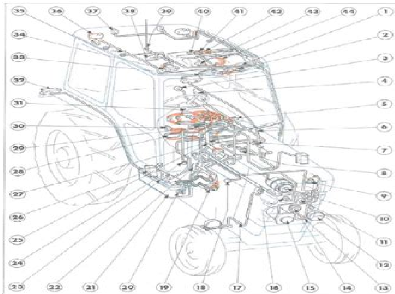
Figure 4 Electrical System—Ford 6700 and 7700—With Flat Deck Cab—4 or 6 Feet
