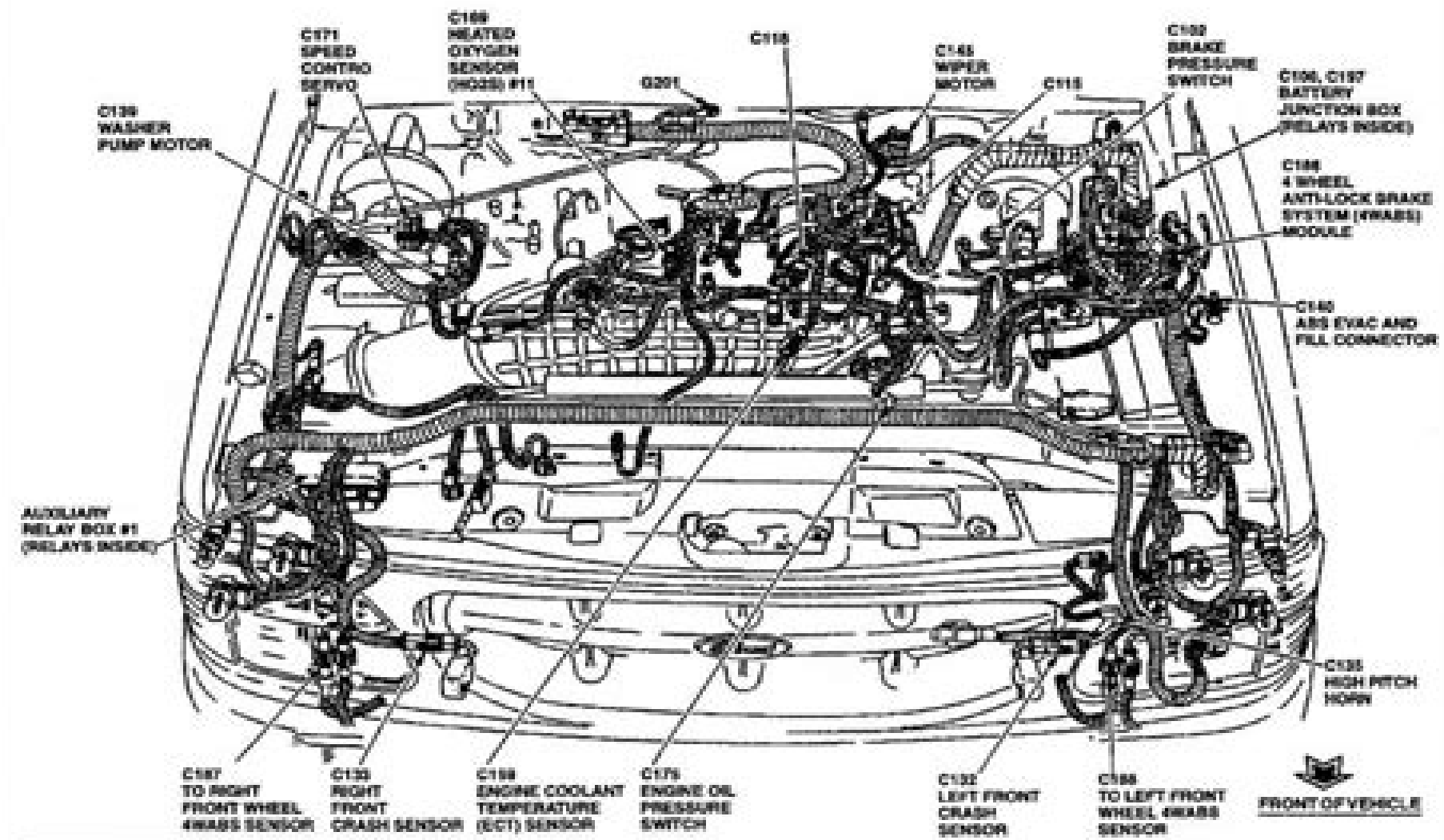
Fig 1: Engine Compartment (4.0L - DOHC)
