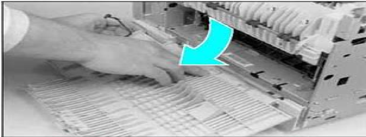
Figure 6-7a Releasing the Door Hinge (LaserJet 4/5)
