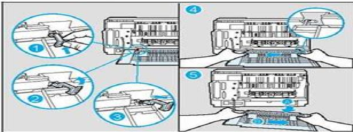
Figure 6-7b Releasing the Door Hinge (LaserJet 4 Plus)
