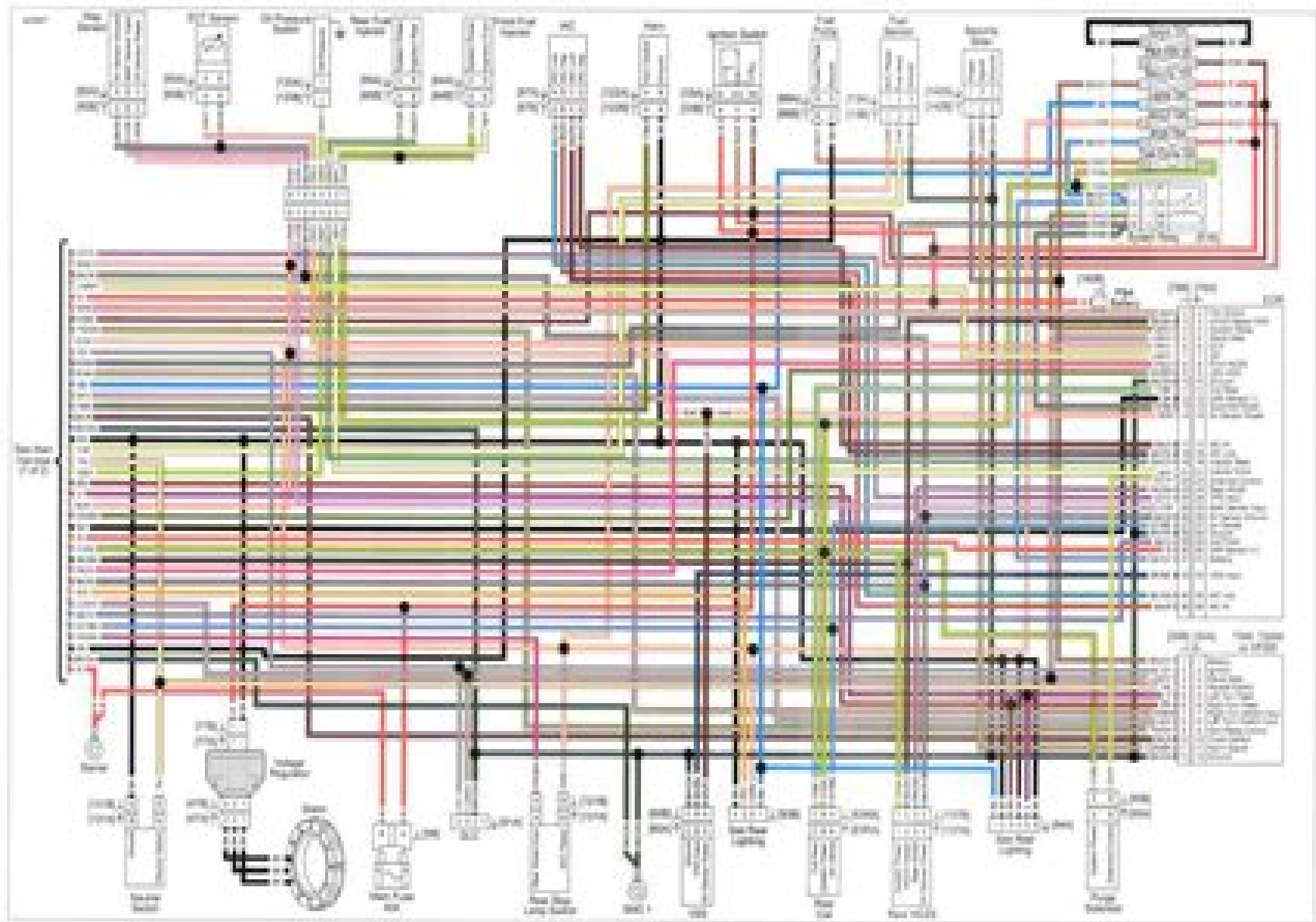
Figure 3-14. Main harness (2 of 2) (2010 model)
