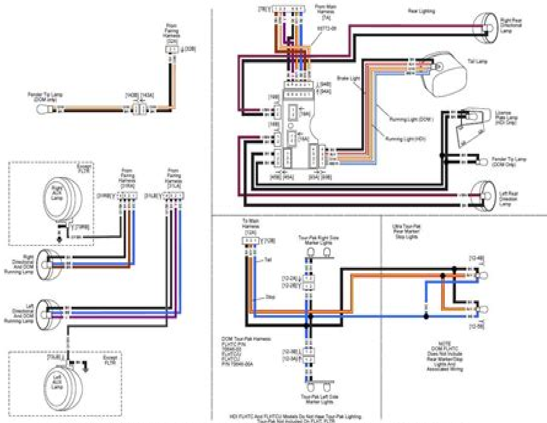
Figure B-27: TAIL, LAMP, AUXILIARY LAMPS, DIRECTIONAL LAMPS, & TOUR/PARK LAMPS - 2008 FLHT, FLHX, FLHTC, FLHTCU, & FLTR DOMESTIC & INTERNATIONAL MODELS
