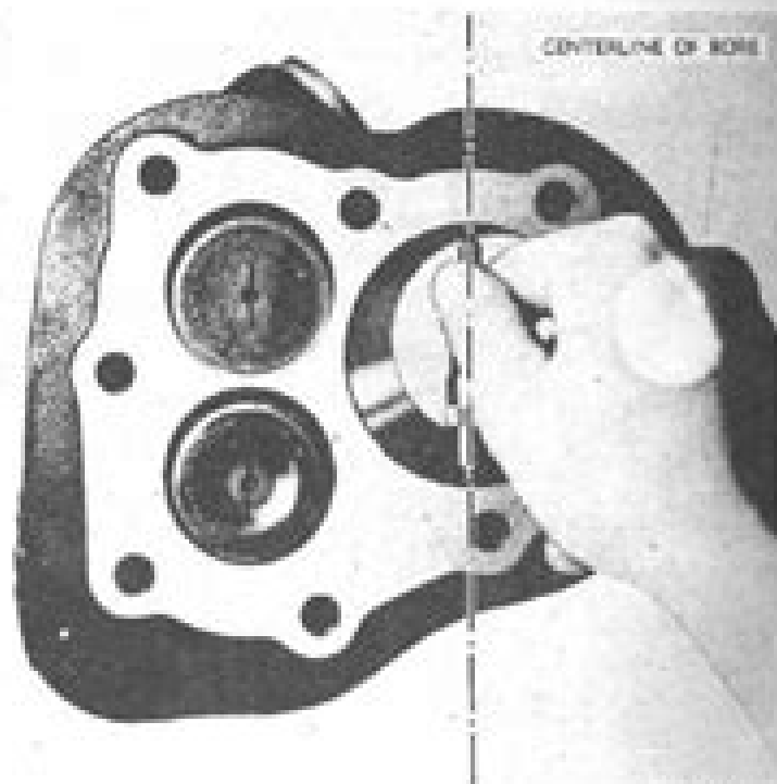
Figure 9—Measuring Cylinder Bore One-half Inch From Top, with Inside Calipers (81-C-304)
