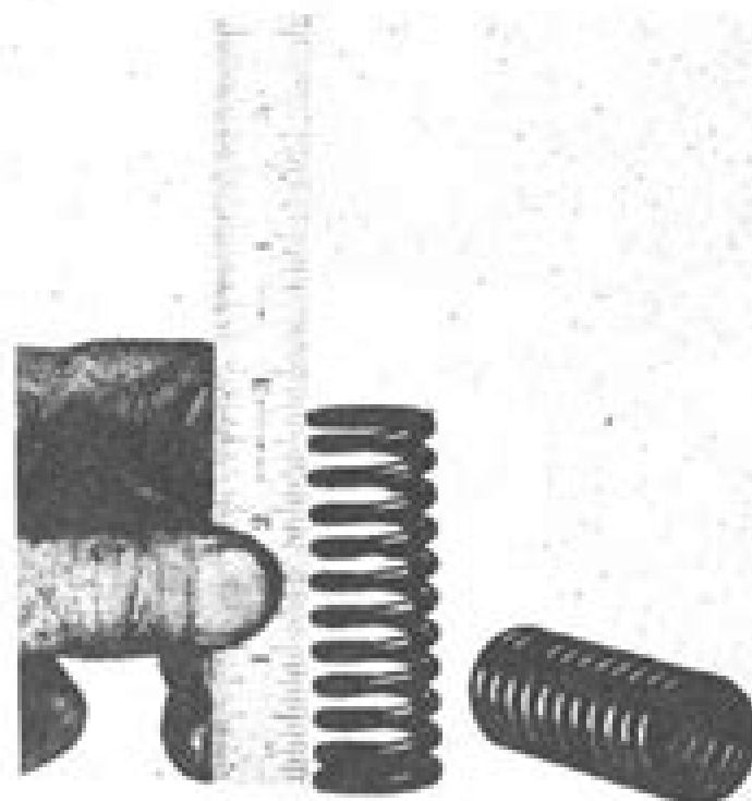
Figure 10—Measuring Length of Valve Springs
