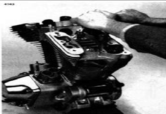
Figure 3-15. Loosen Cylinder Head Bolts
