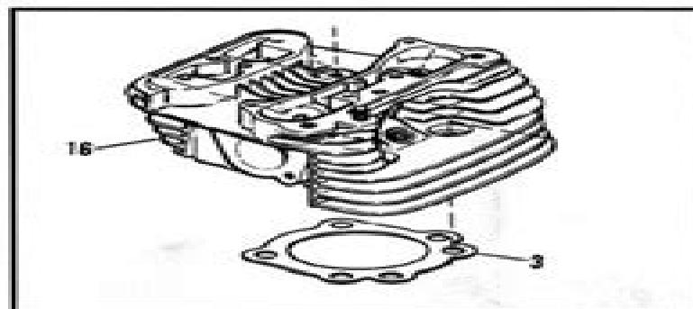
Figure 3-17. Cylinder Head and Gasket
