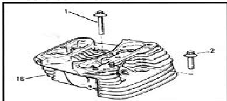
Figure 3-16. Cylinder Head Bolts
