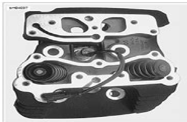
Figure 3-2. Spring/Valve Stack and ACR
