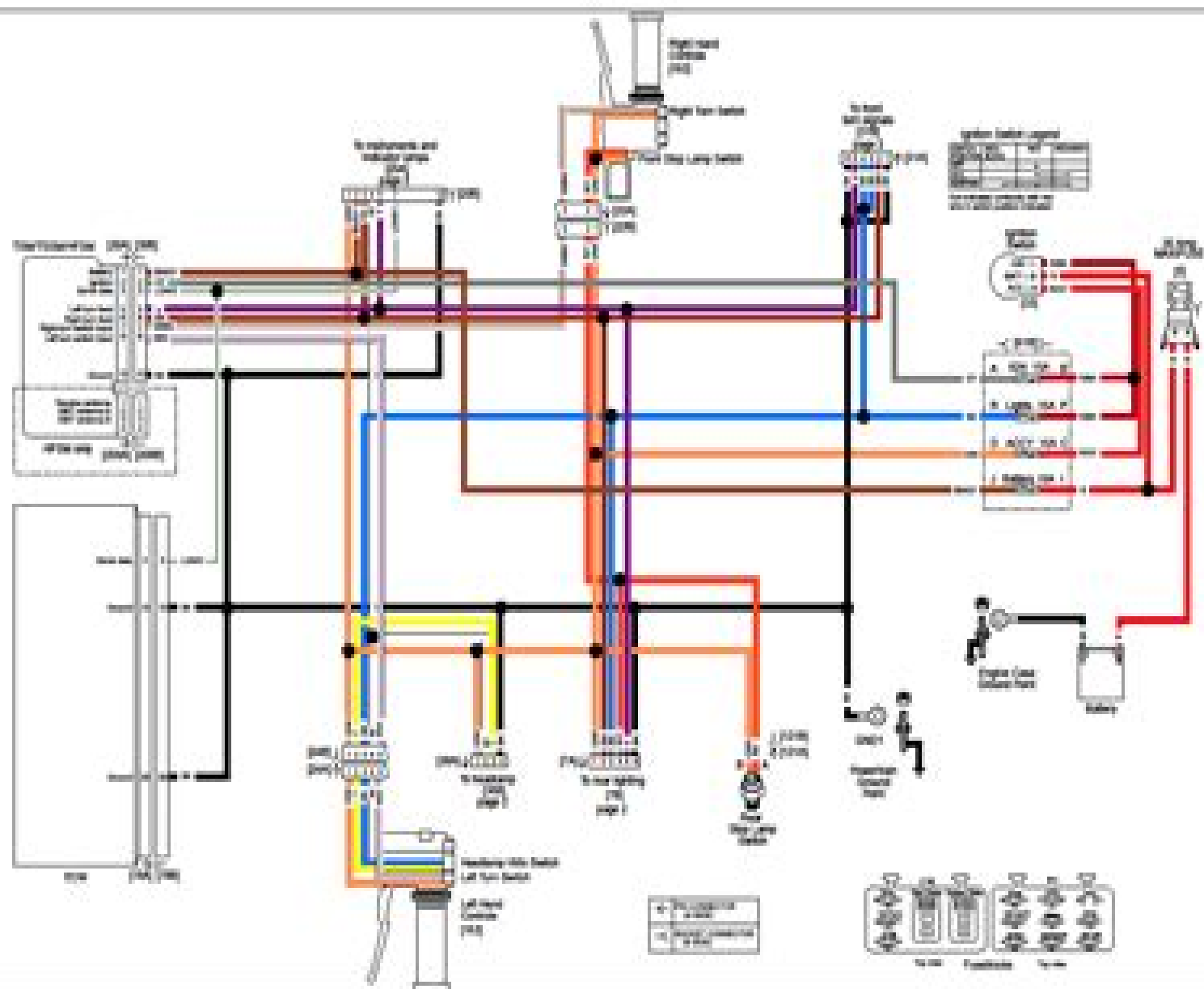
Figure 9-2: Lights (1 of 2) (DL) 2000 Spectra DM and RW Models
