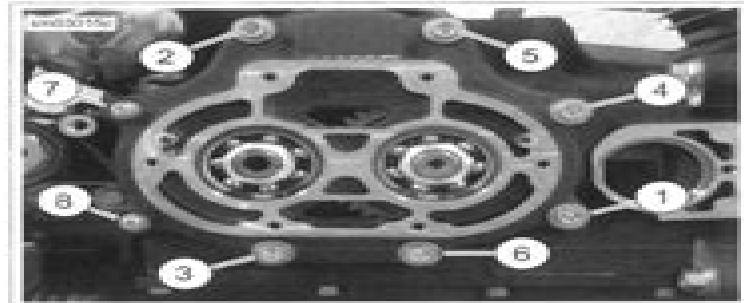
Figure 6-34. Torque Sequence
