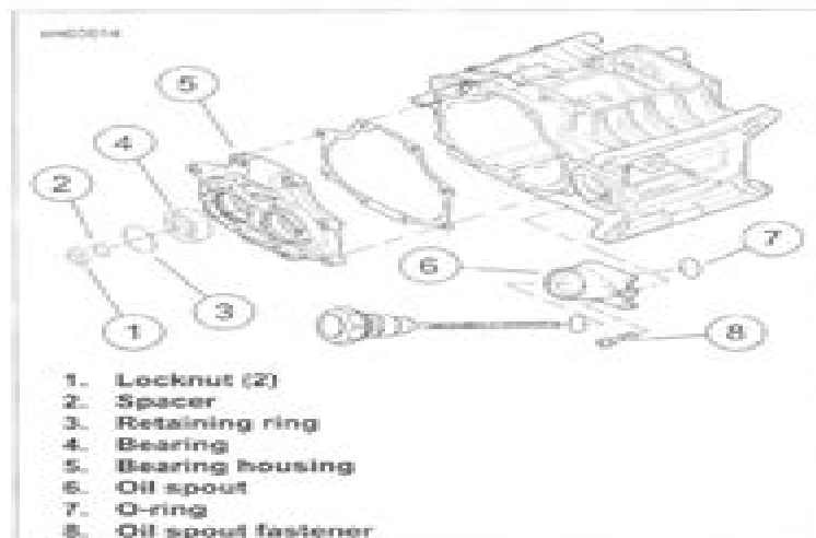
Figure 6-35. Bearing Housing Bearings
