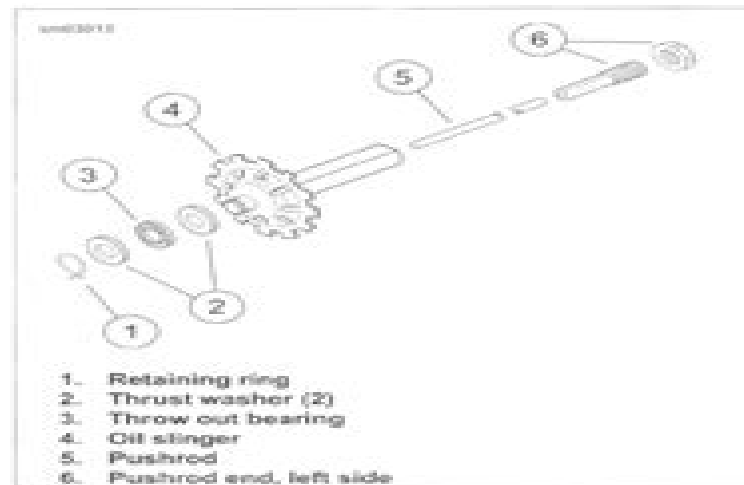
Figure 6-36. Pushrod Assembly: Cable Clutch
