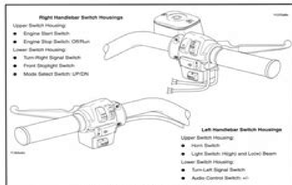
Figure 9-116. Classic Handlebar Switch Assemblies
