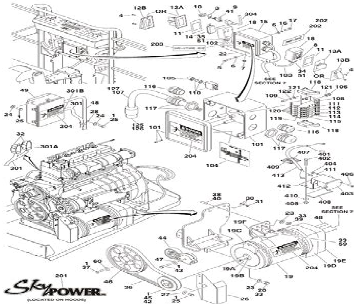
FIGURE 2-21. 7500W SKYPOWER GENERATOR INSTALLATION
