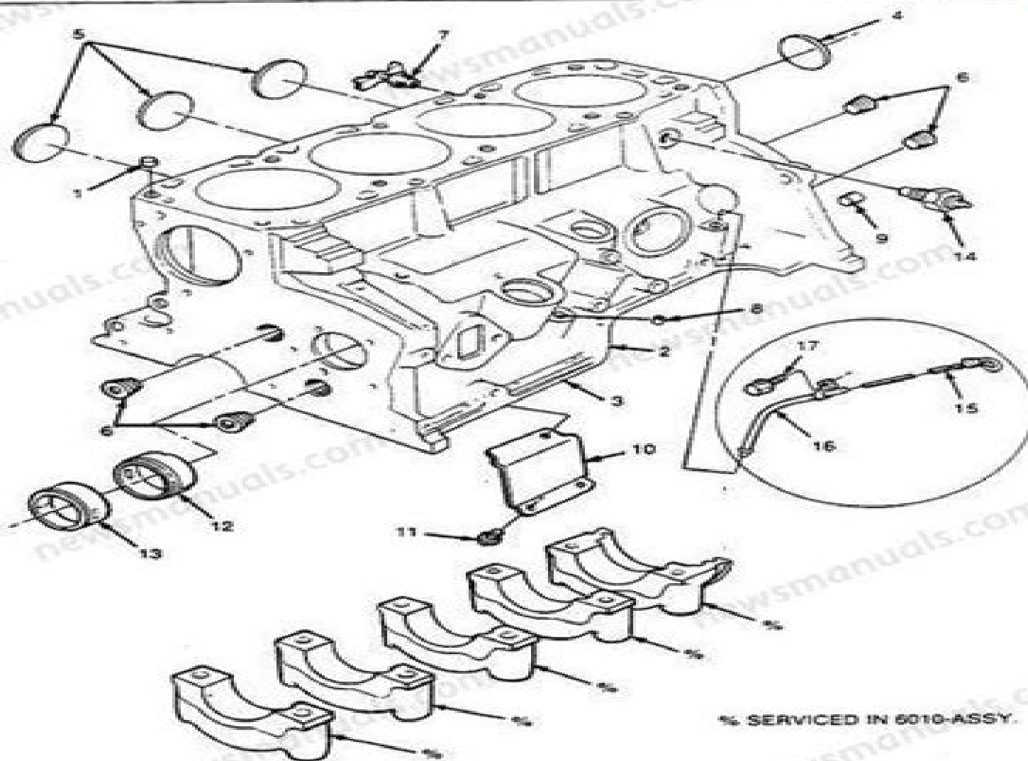
CYLINDER BLOCK AND RELATED PARTS — TYPICAL
