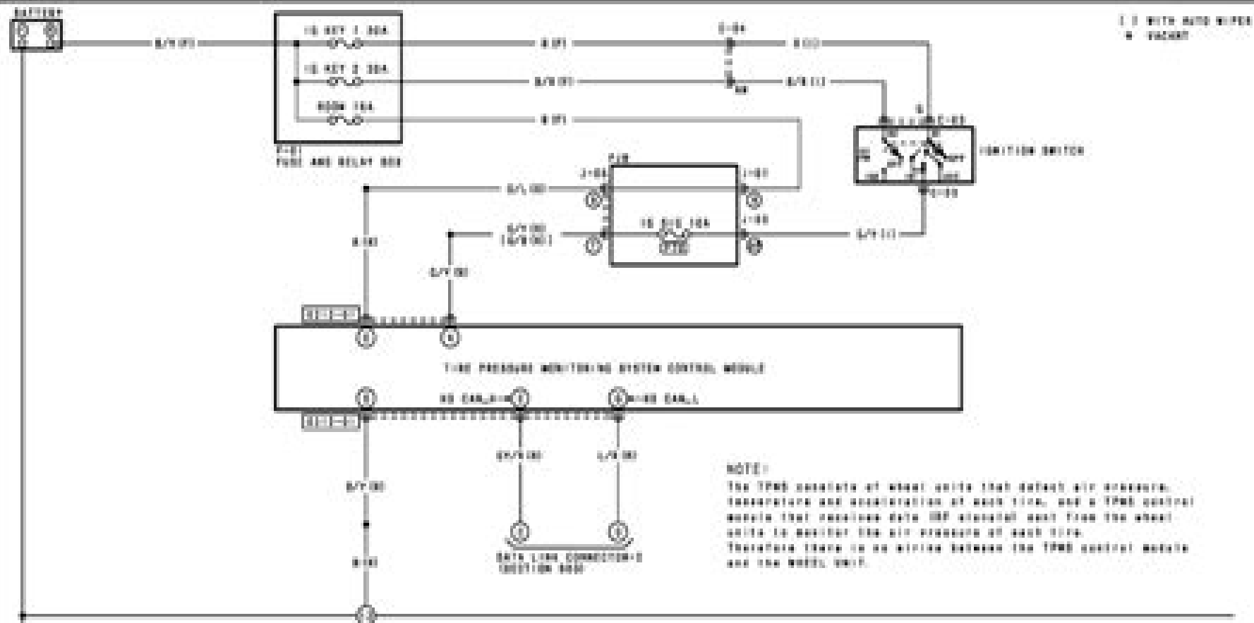
TPMS MONITORING SYSTEM CONTROL MODULE (M)
