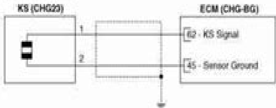
[Harness Connector]
