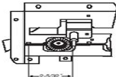
Fig. 14 - Igniter
