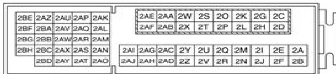
PCM WIRING HARNESS-SIDE CONNECTOR
