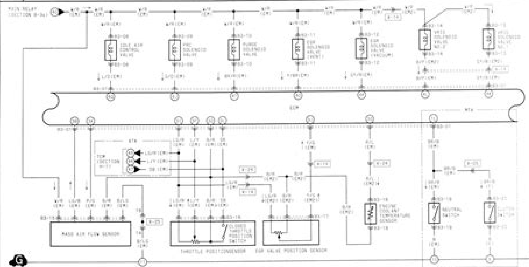
B-3-01 EGR VALVE
