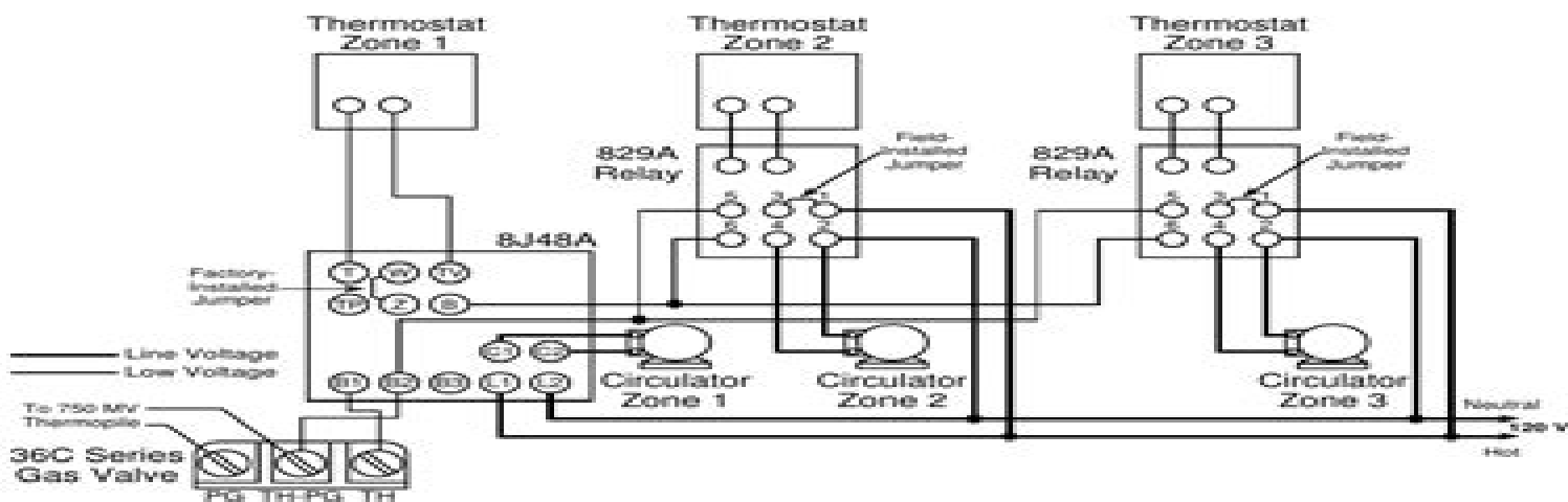
Figure 9. 8J48A - Millivolt Systems Zoned with Circulators
