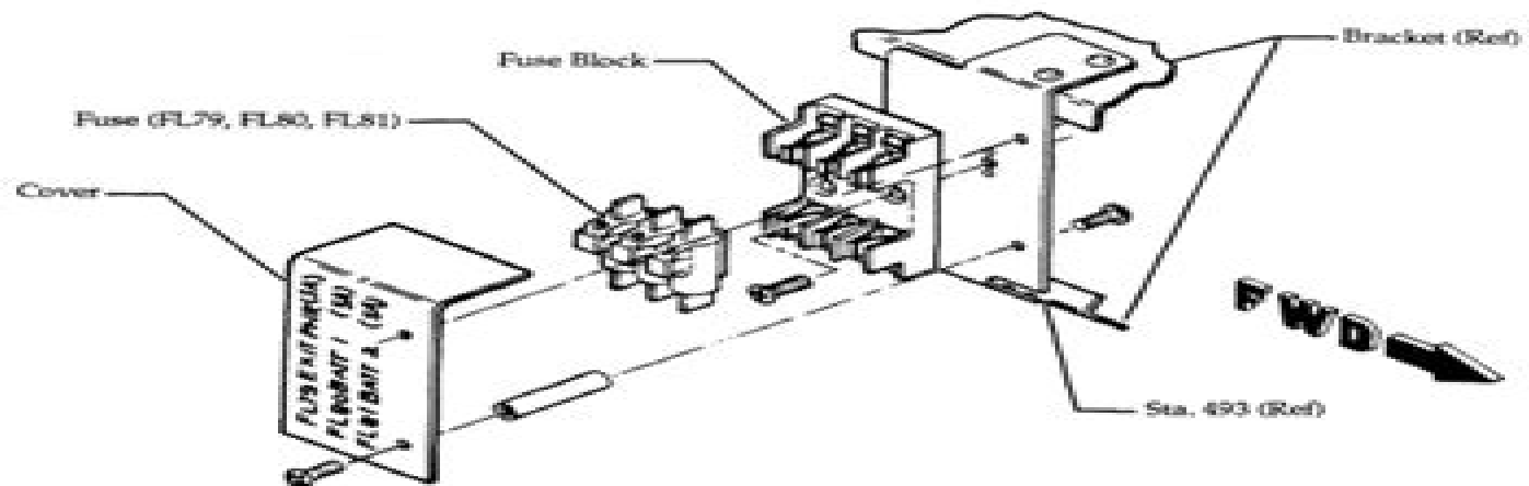
External Power Receptacle Fuse Installation Figure 202
