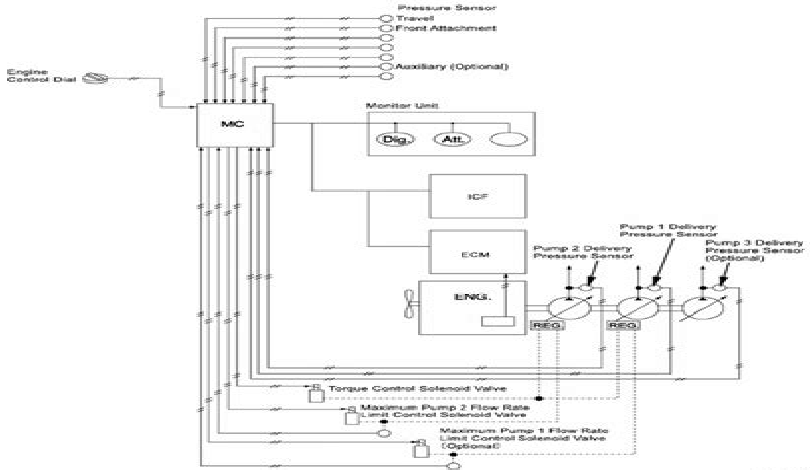
Pump Control System Layout
