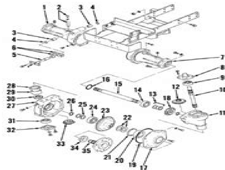
Fig. 9—Exploded view of four-wheel drive front axle assembly available on Models 244 and 254.
