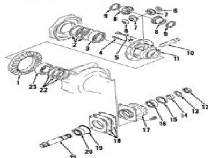
Fig. 8—Exploded view of four-wheel drive front differential used on Model 234.
