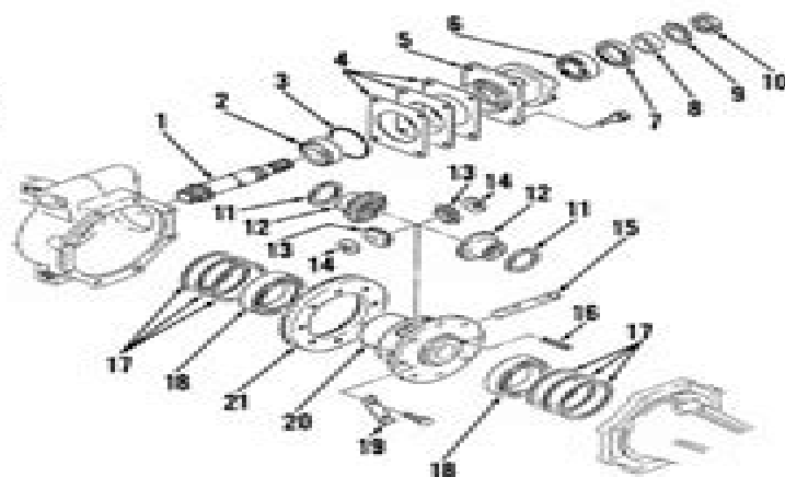
Fig. 10—Exploded view of four-wheel drive front differential used on Models 244 and 254.
