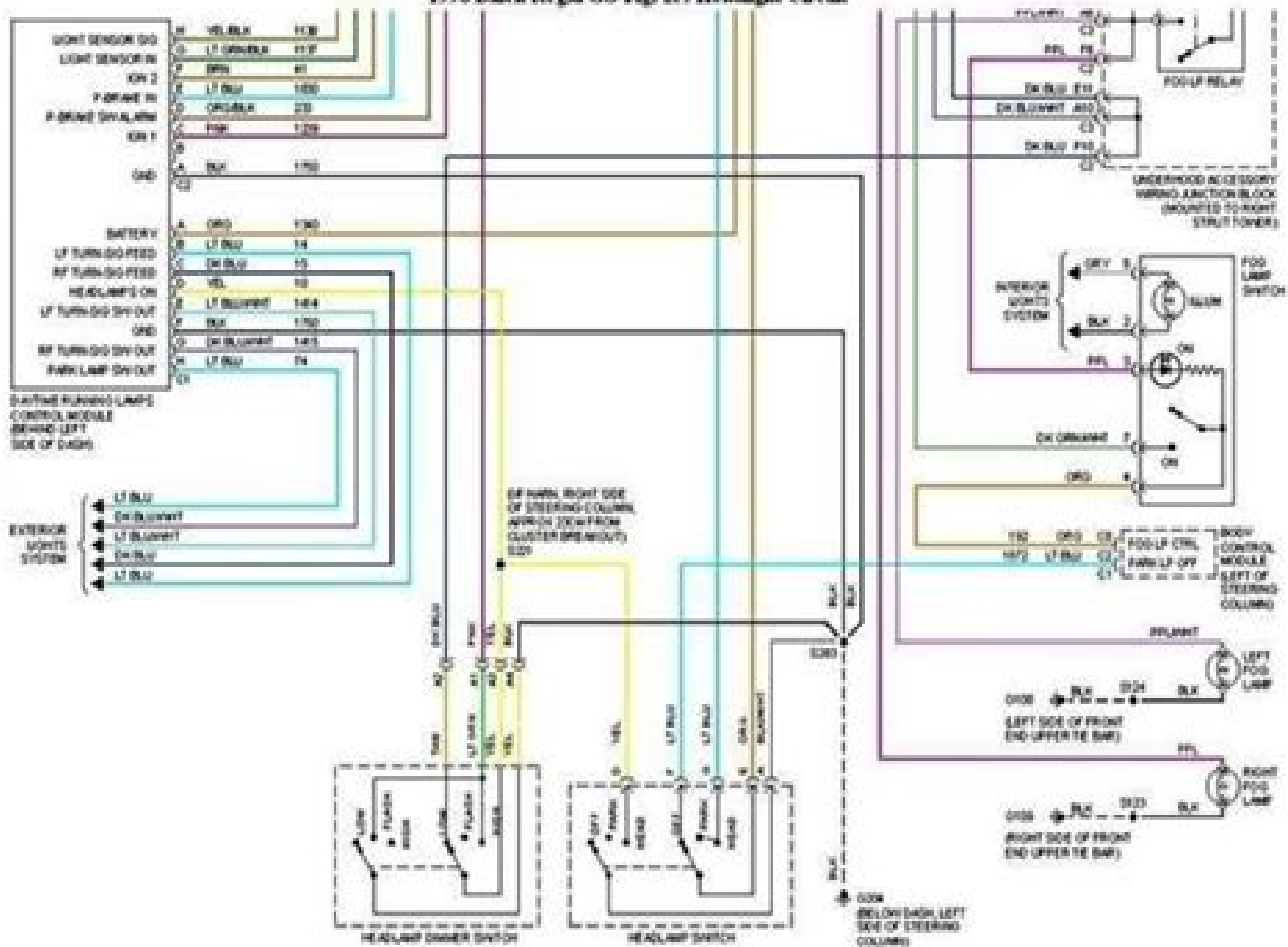
1998 Buick Regal GS-Fig. 15: Headlight Circuit
