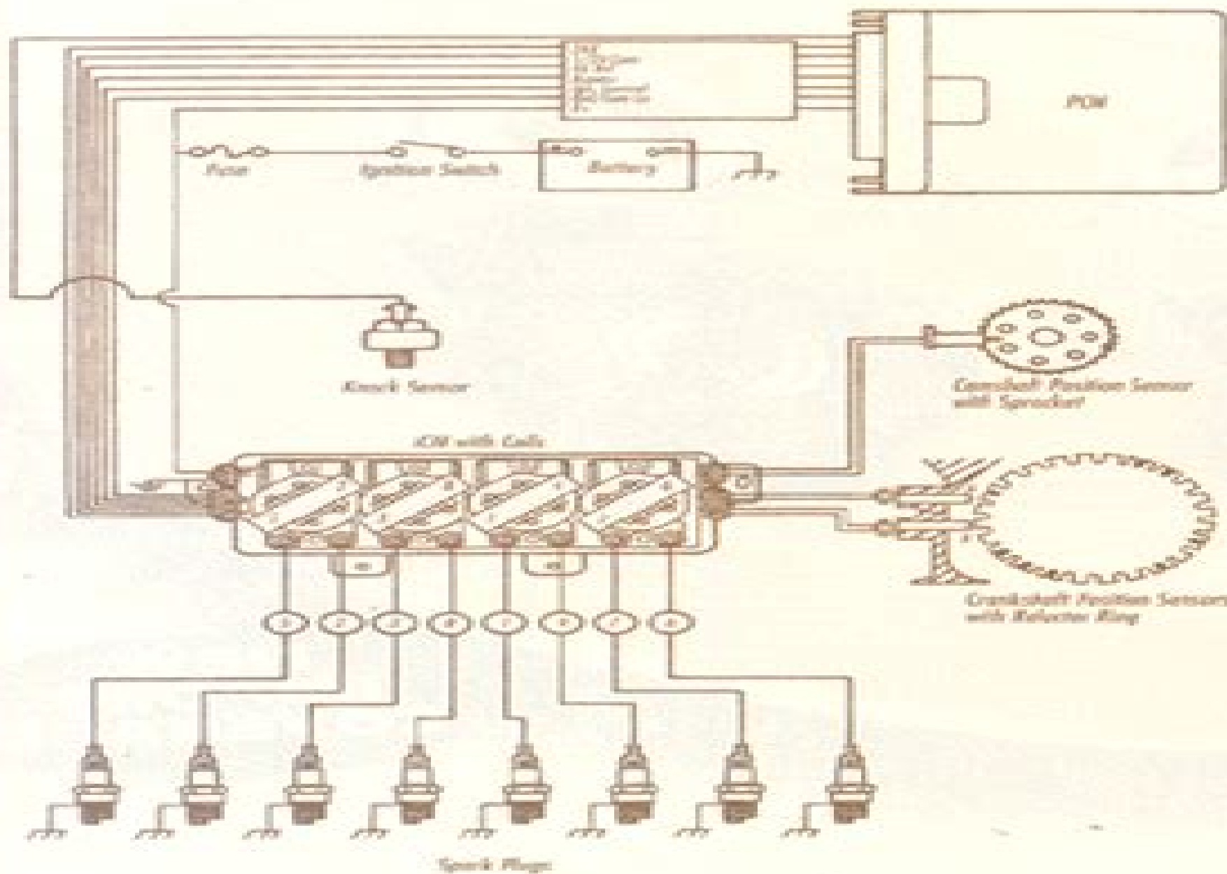
1993-'99 Northstar V8 ignition system
