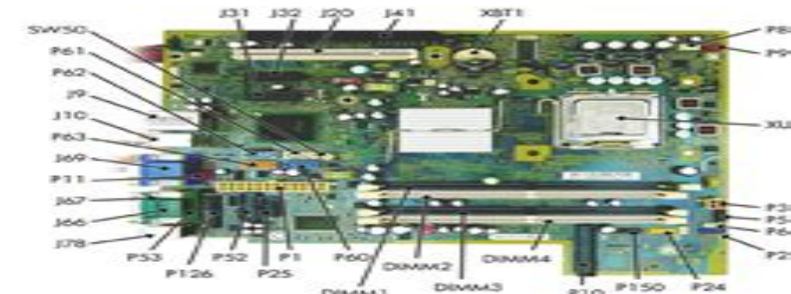
System Board Connectors and Jumpers (position of some unfilled components may vary in location)
