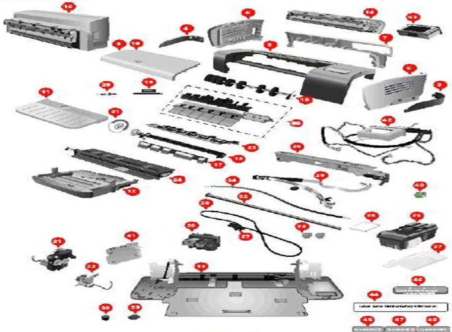
Exploded view
