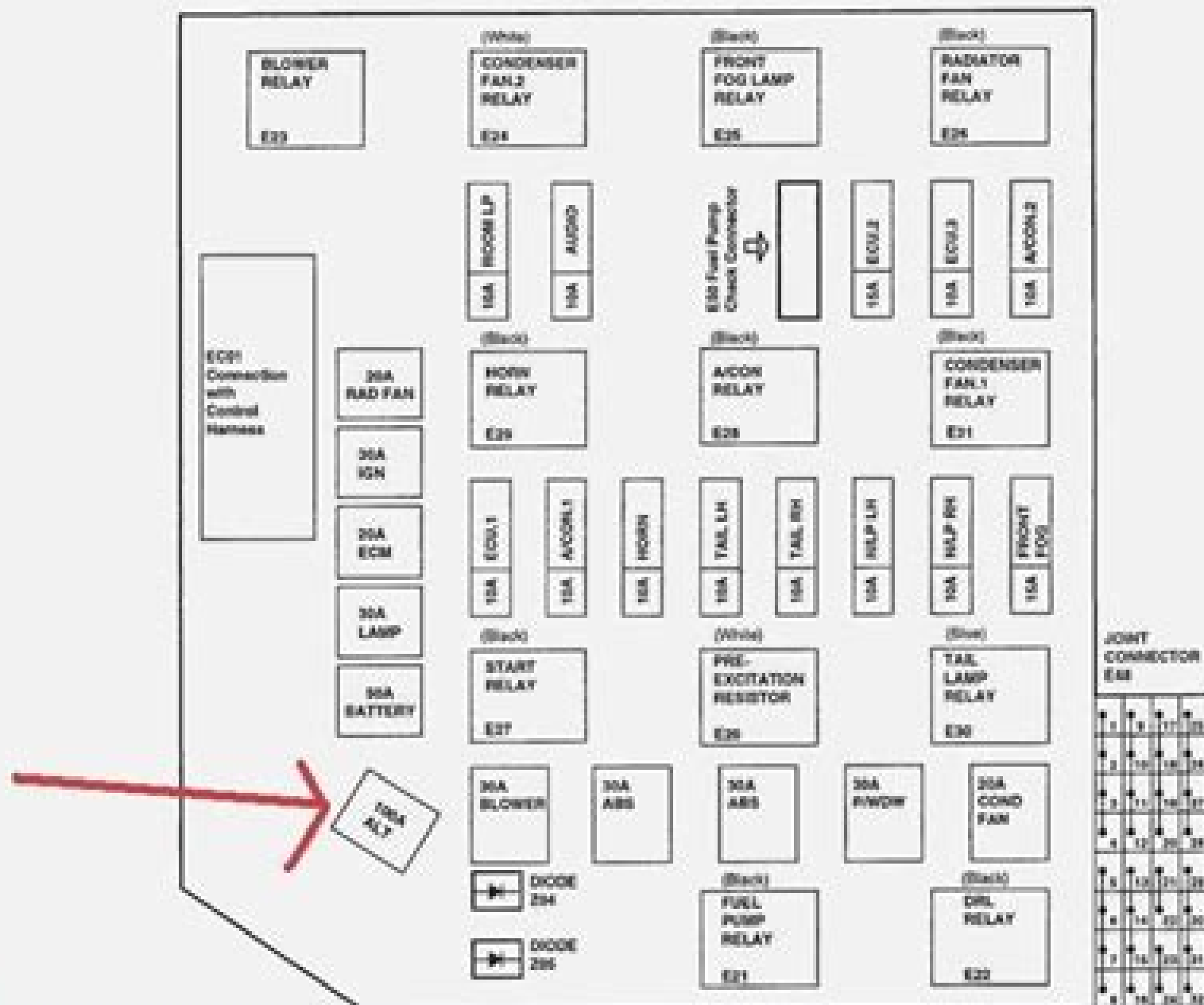
Fig. 7: Identifying Engine Compartment Relay & Fuse Box Components
