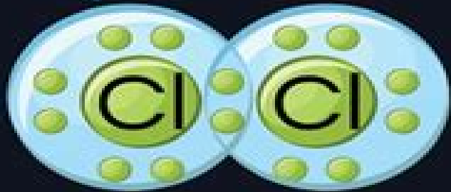
Nonpolar covalent
