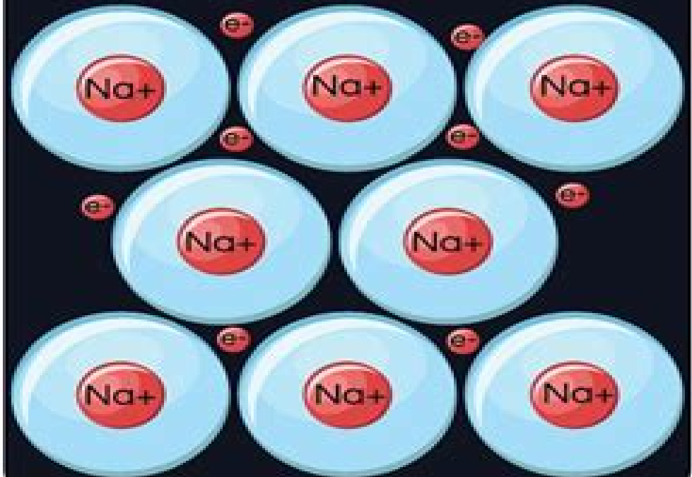
Metallic
