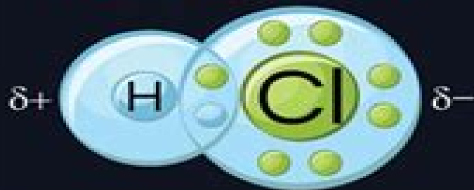
Polar covalent
