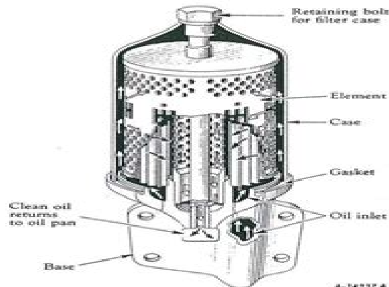
Illustr. 29 Cutaway view of the oil filter showing the passage of oil through the inside and outside surfaces of the filter element.
