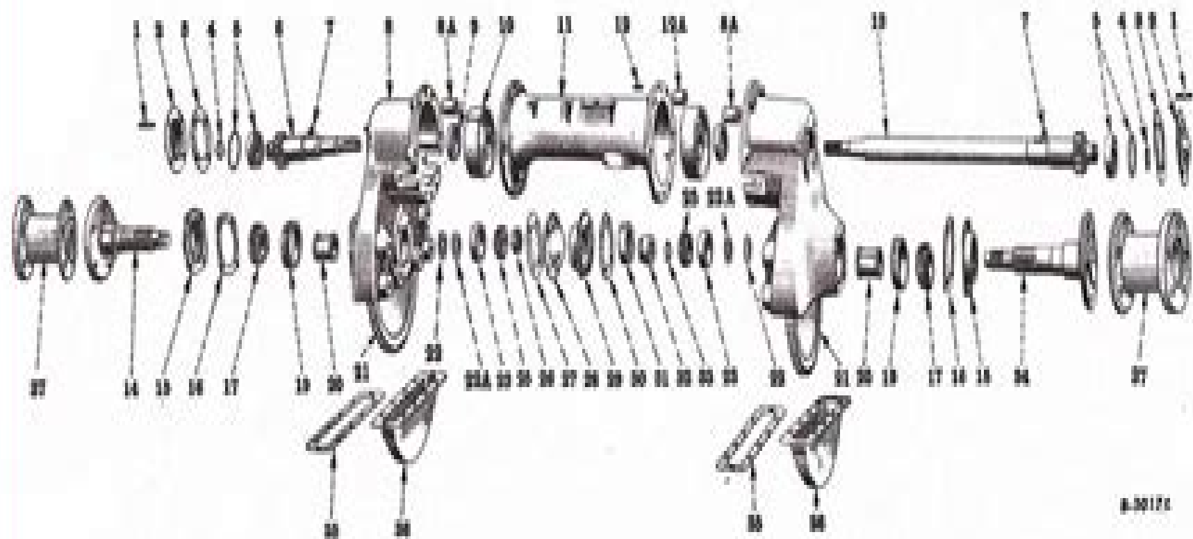
FINAL DRIVE
