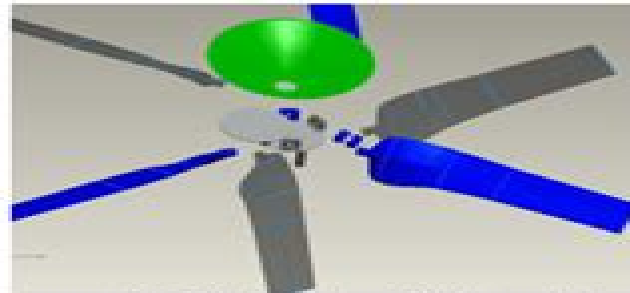
Fig.-2. Exploded view of The fan assembly
