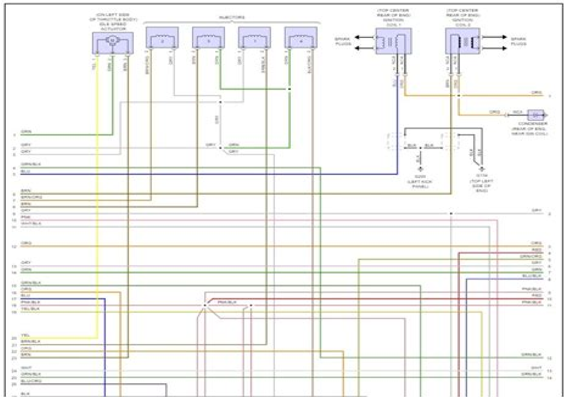
Fig 2: 1.6L, Engine Performance Circuits (2 of 3)
