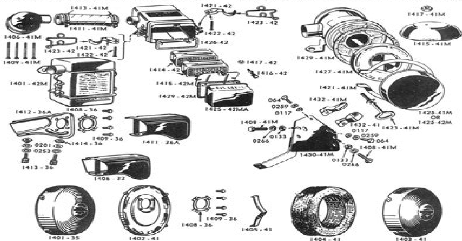
AIR INTAKE AND CLEANERS
