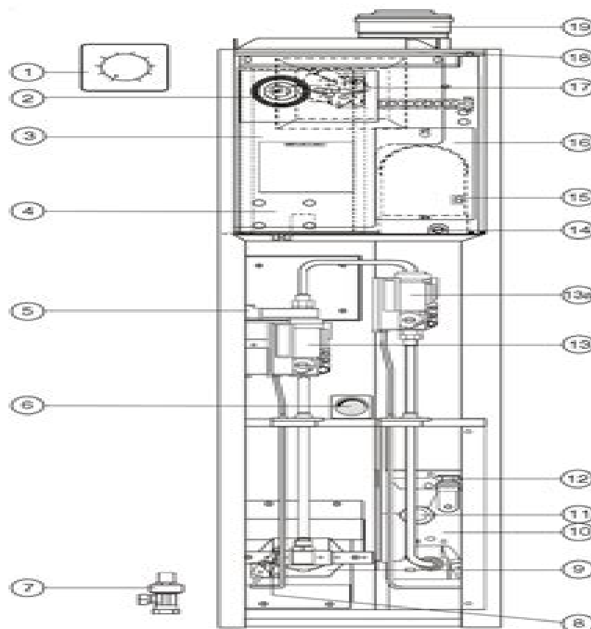
Fig. 1 Heater with Sealing Panel removed
