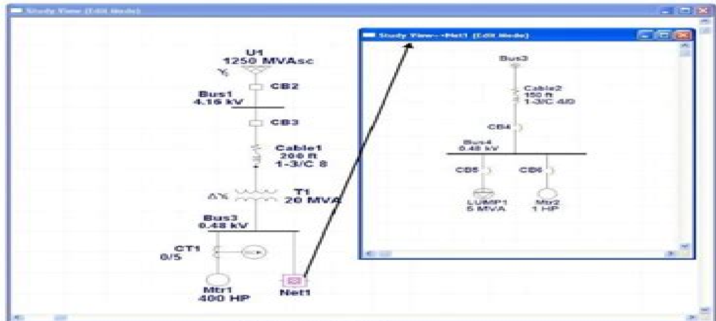
Final one-line diagram
