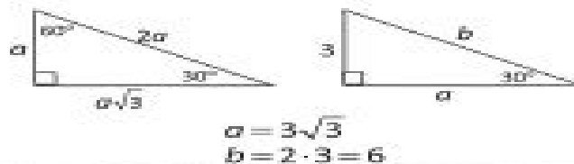
30-60-90 Triangle
